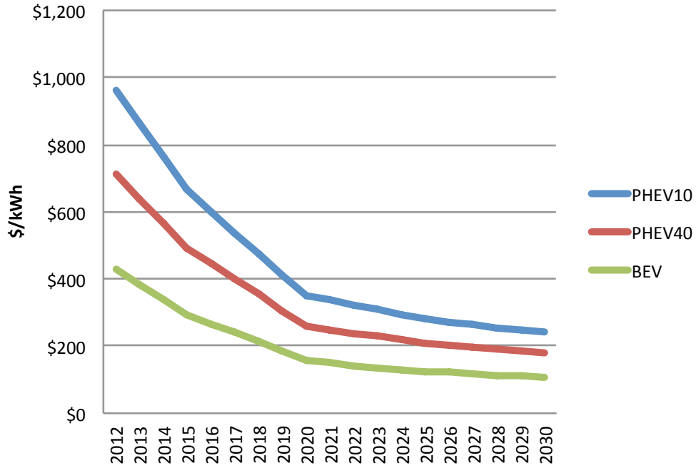
Figure 3.7: Battery Cost/Efficiency, by Vehicle Type
